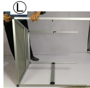
3: Insert the alu tube with two grooves into the panel at the bottom corner
