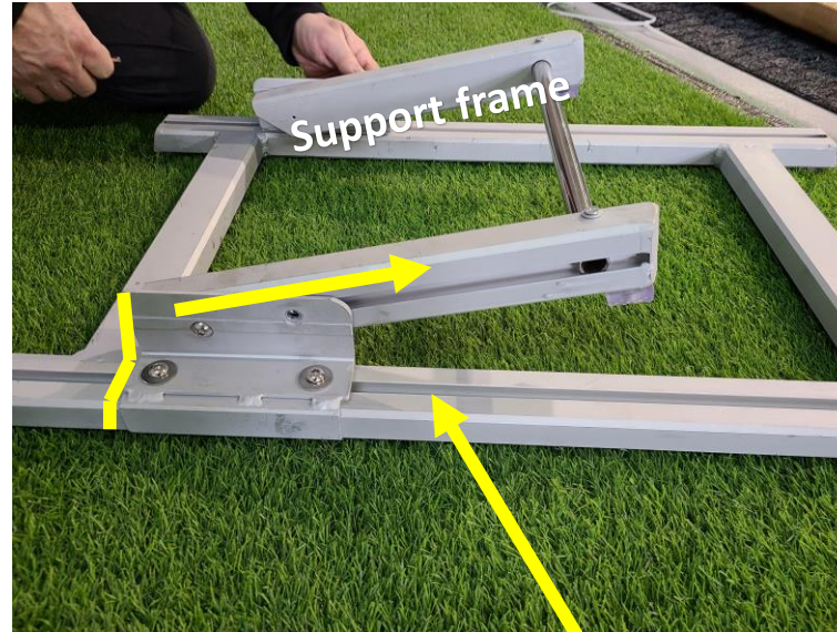
Place the teeter base with slots facing up as shown on a smooth flat surface and using the bolts and washers provided attach the brackets as shown above using a metric hex key
